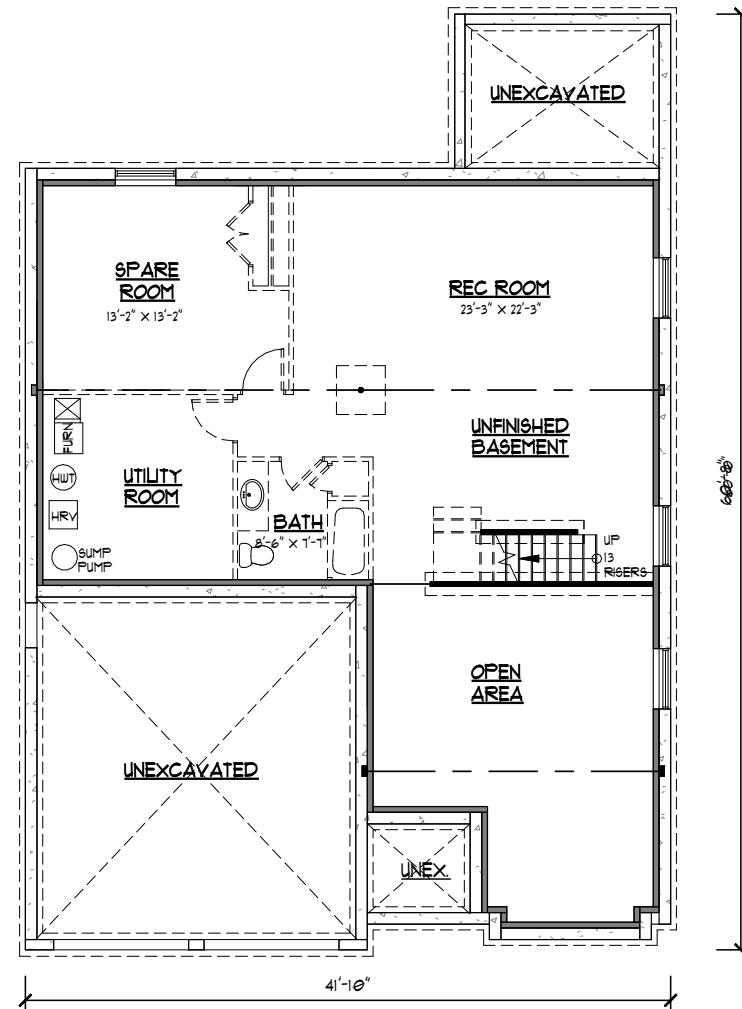
OPTIONAL BASEMENT FLOOR PLAN
